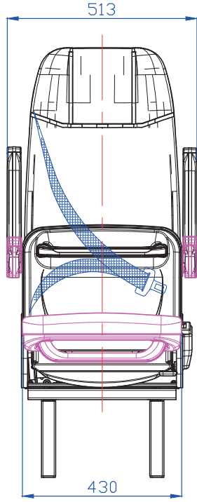
TECHNICAL DRAWING (FRONT VIEW)
