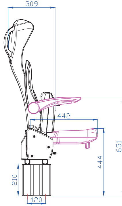
TECHNICAL DRAWING (SIDE VIEW)
